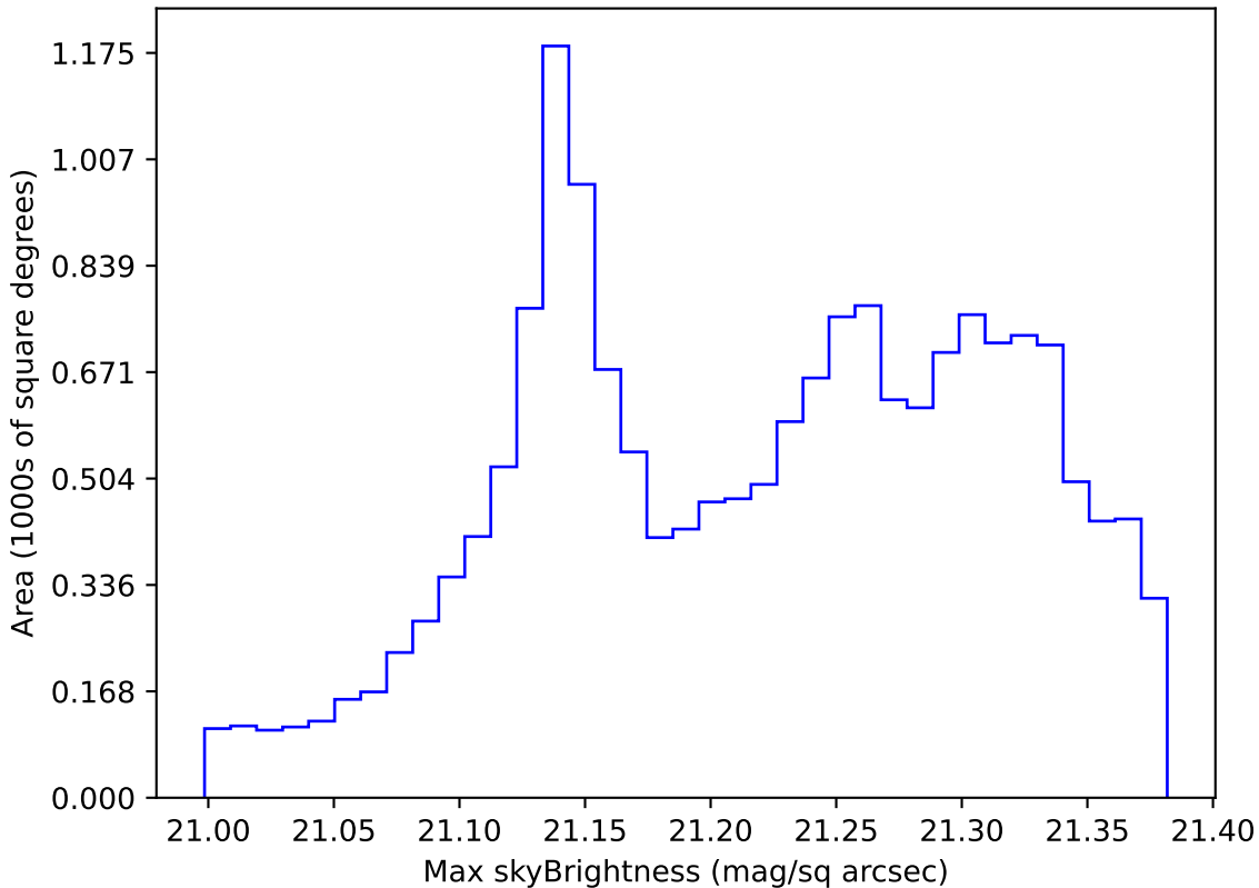
too_ignore_10_1v3.4_10yrs WFD r band: Max skyBrightness
