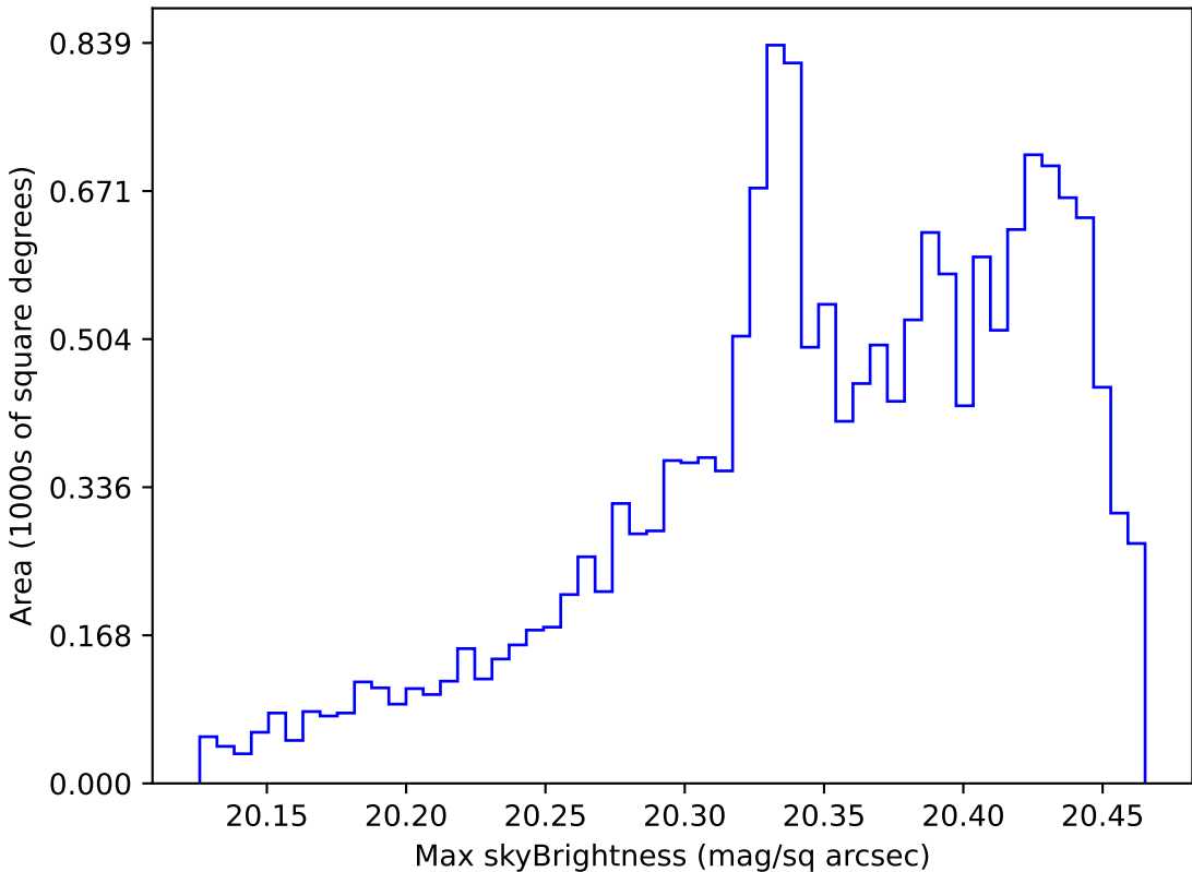
too_ignore_10_1v3.4_10yrs WFD i band: Max skyBrightness
