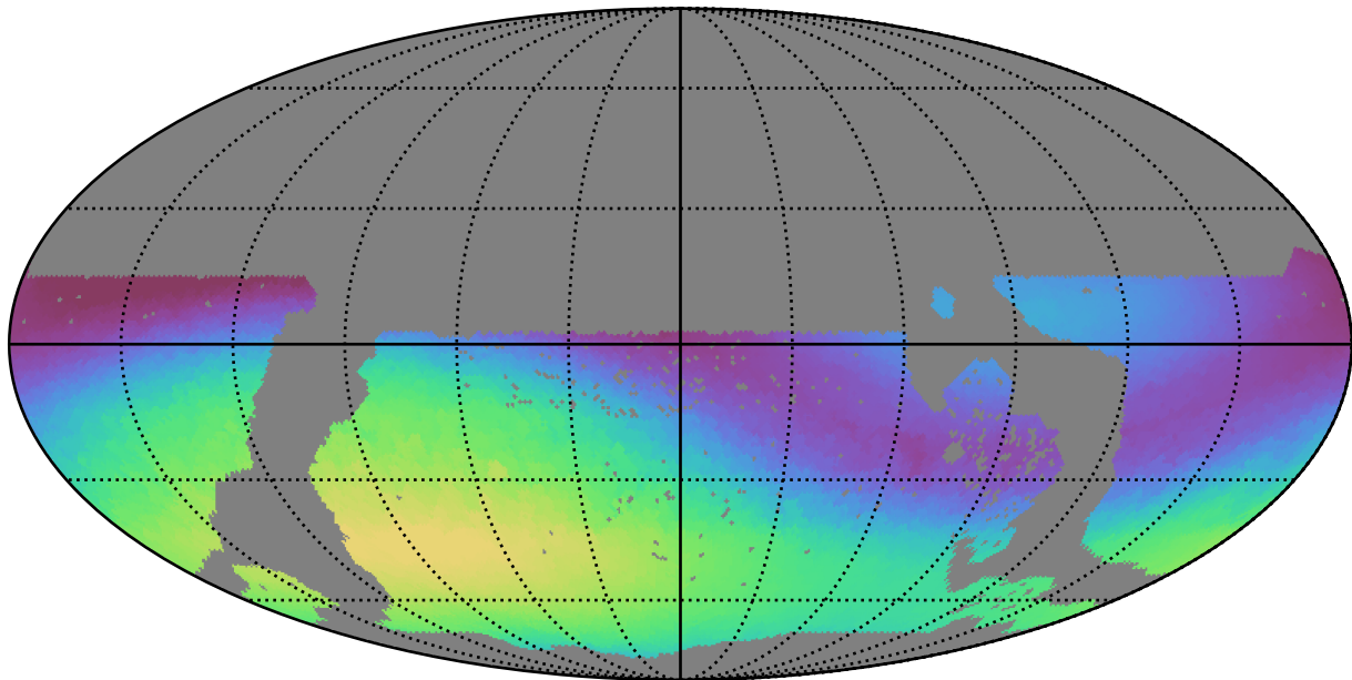
too_ignore_10_1v3.4_10yrs WFD g band: Max skyBrightness
