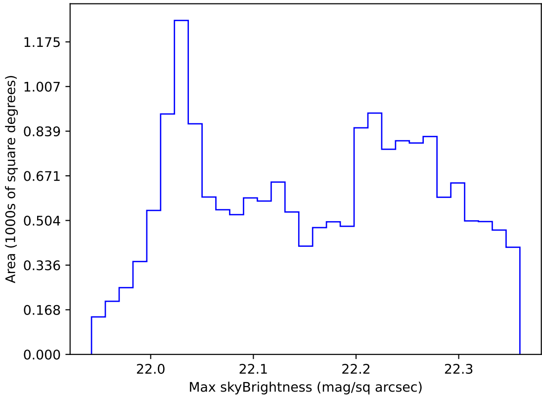
too_ignore_10_1v3.4_10yrs WFD g band: Max skyBrightness
