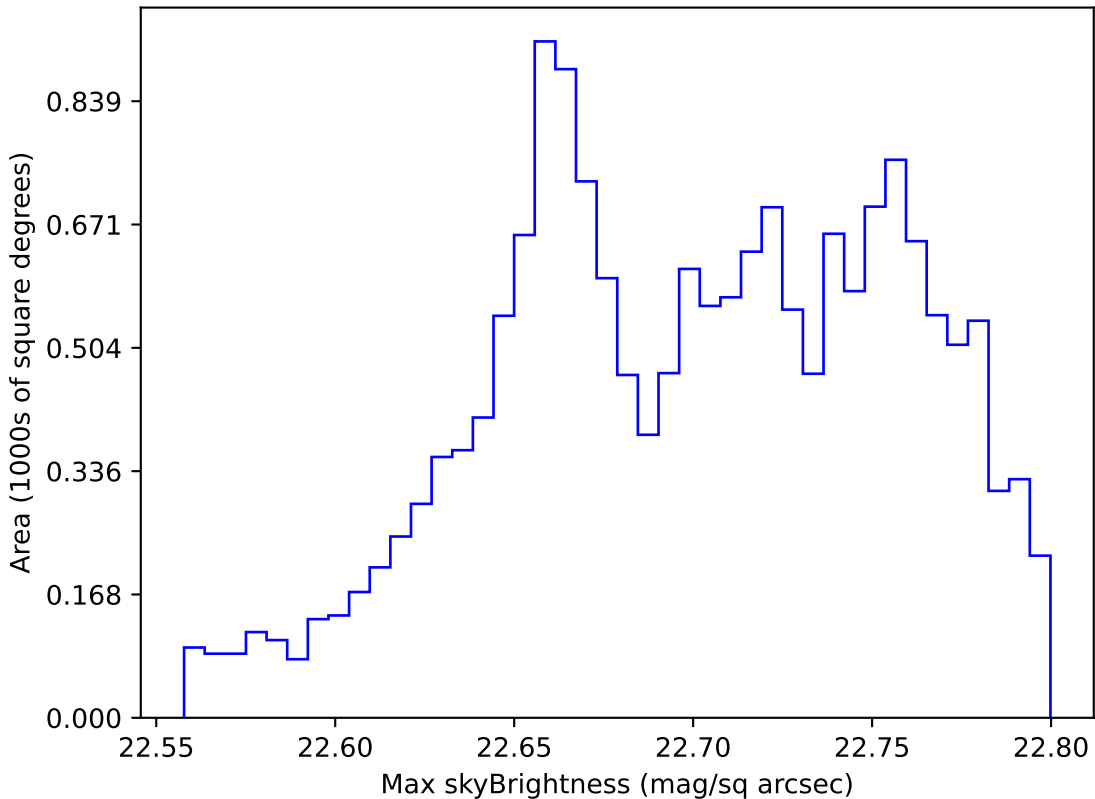
too_ignore_10_1v3.4_10yrs WFD all bands: Max skyBrightness
