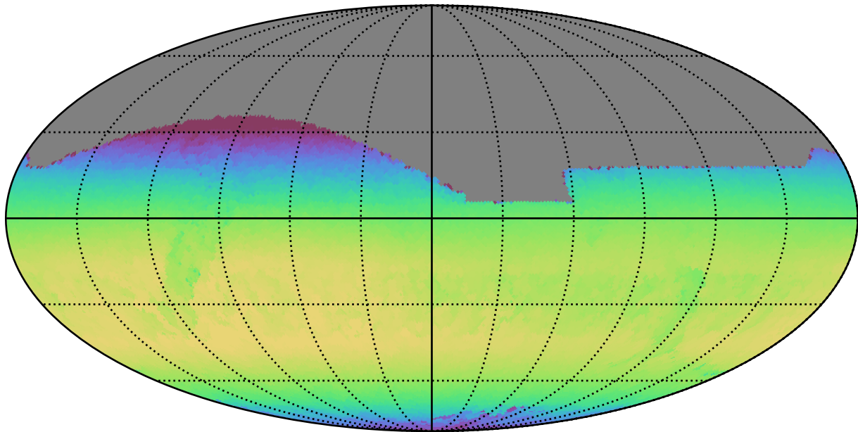
too_ignore_10_1v3.4_10yrs All sky z band: Max skyBrightness
