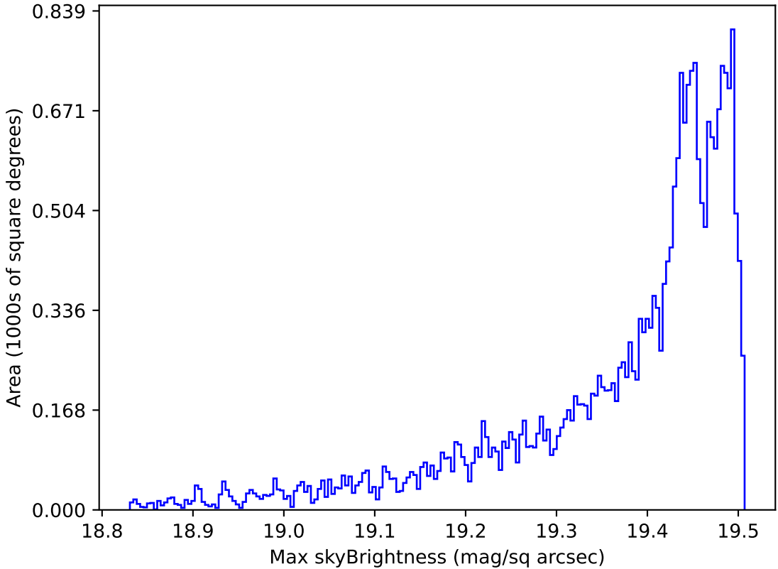
too_ignore_10_1v3.4_10yrs All sky z band: Max skyBrightness
