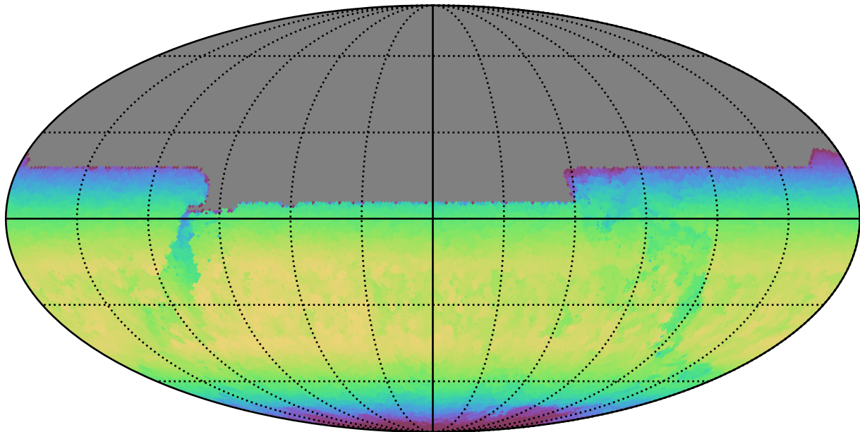
too_ignore_10_1v3.4_10yrs All sky y band: Max skyBrightness
