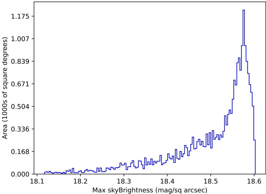
too_ignore_10_1v3.4_10yrs All sky y band: Max skyBrightness
