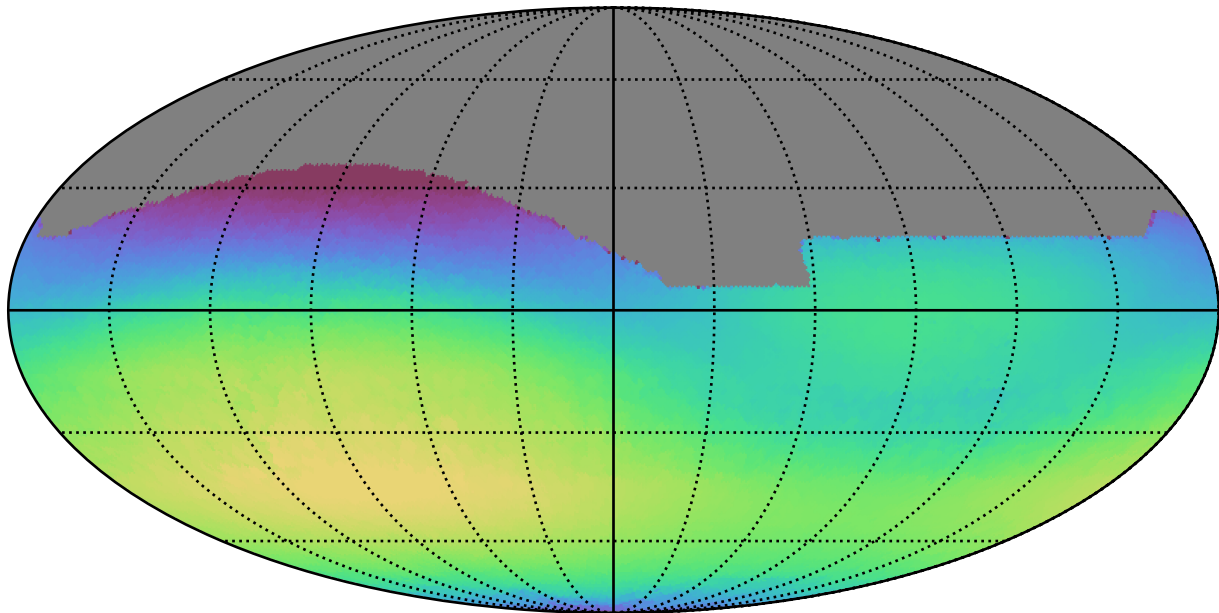
too_ignore_10_1v3.4_10yrs All sky r band: Max skyBrightness
