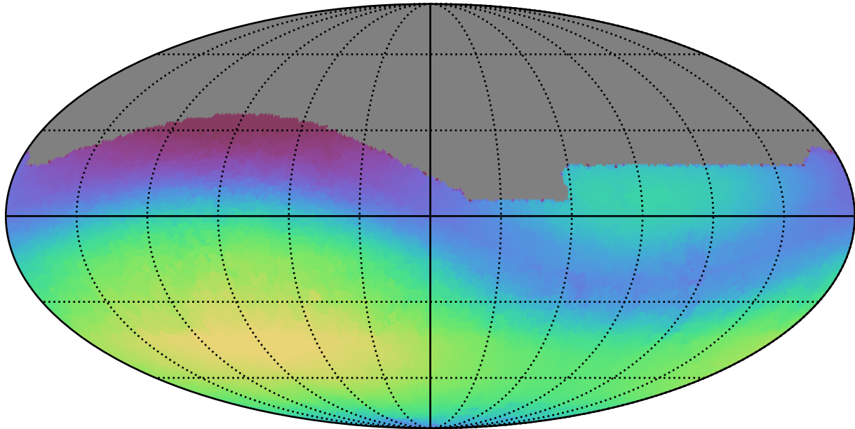
too_ignore_10_1v3.4_10yrs All sky g band: Max skyBrightness
