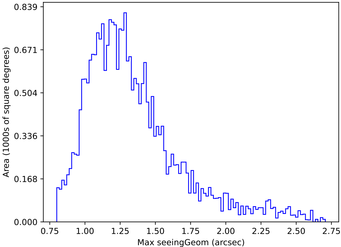
too_ignore_10_1v3.4_10yrs Yr 1 z band: Max seeingGeom
