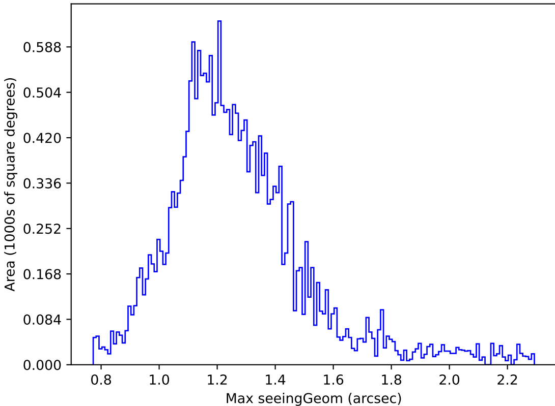
too_ignore_10_1v3.4_10yrs Yr 1 y band: Max seeingGeom
