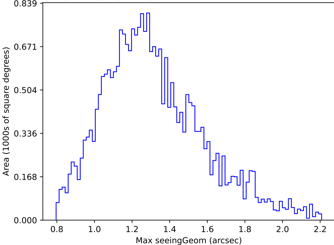
too_ignore_10_1v3.4_10yrs Yr 1 r band: Max seeingGeom
