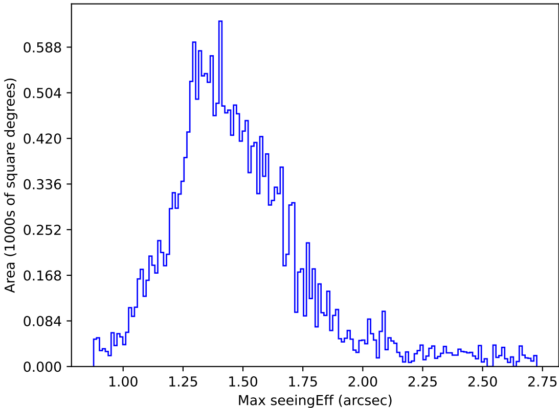
too_ignore_10_1v3.4_10yrs Yr 1 y band: Max seeingEff
