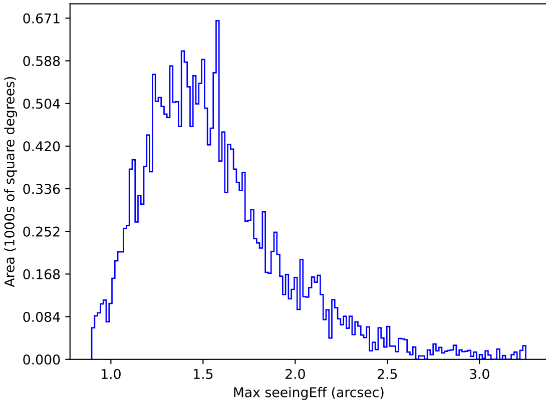
too_ignore_10_1v3.4_10yrs Yr 1 i band: Max seeingEff
