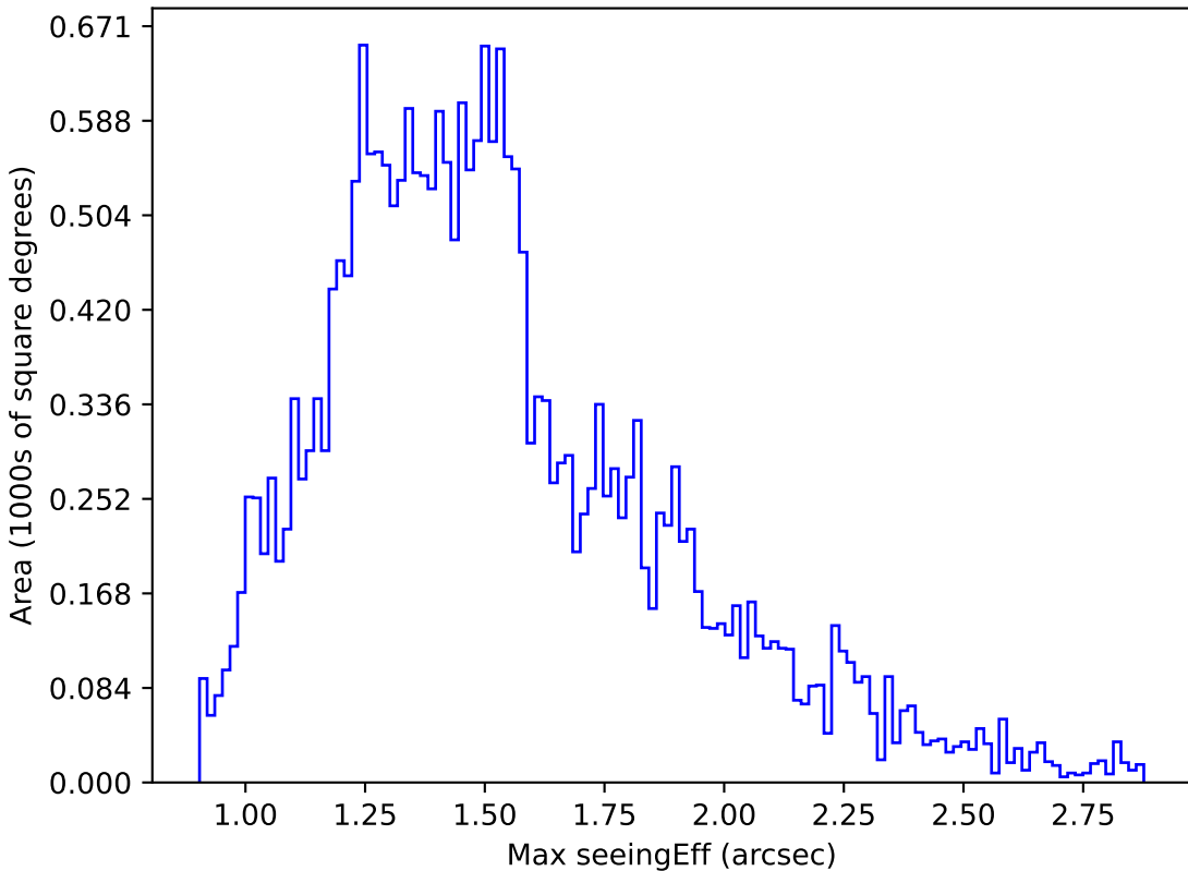
too_ignore_10_1v3.4_10yrs Yr 1 g band: Max seeingEff
