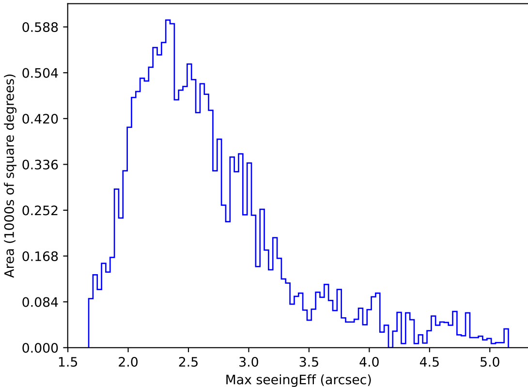
too_ignore_10_1v3.4_10yrs WFD z band: Max seeingEff
