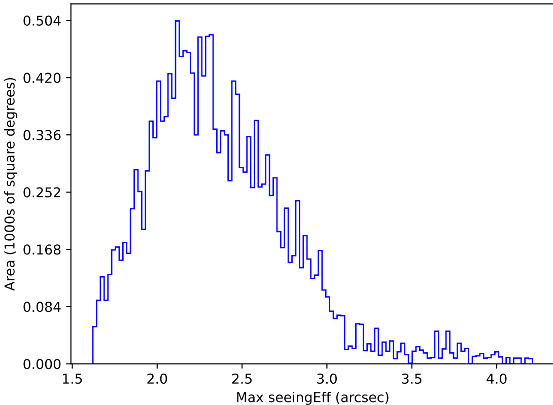
too_ignore_10_1v3.4_10yrs WFD y band: Max seeingEff
