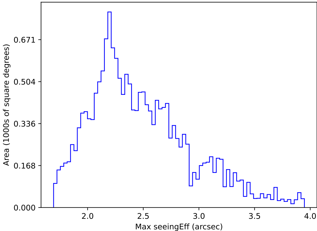
too_ignore_10_1v3.4_10yrs WFD u band: Max seeingEff
