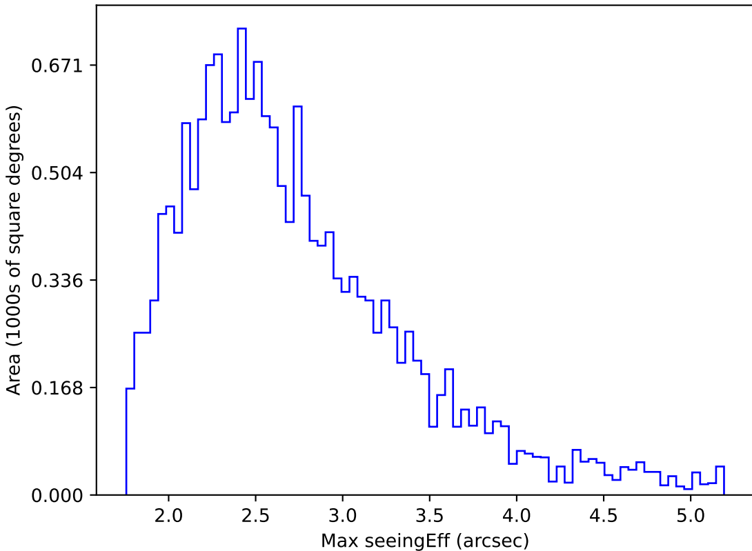
too_ignore_10_1v3.4_10yrs WFD i band: Max seeingEff
