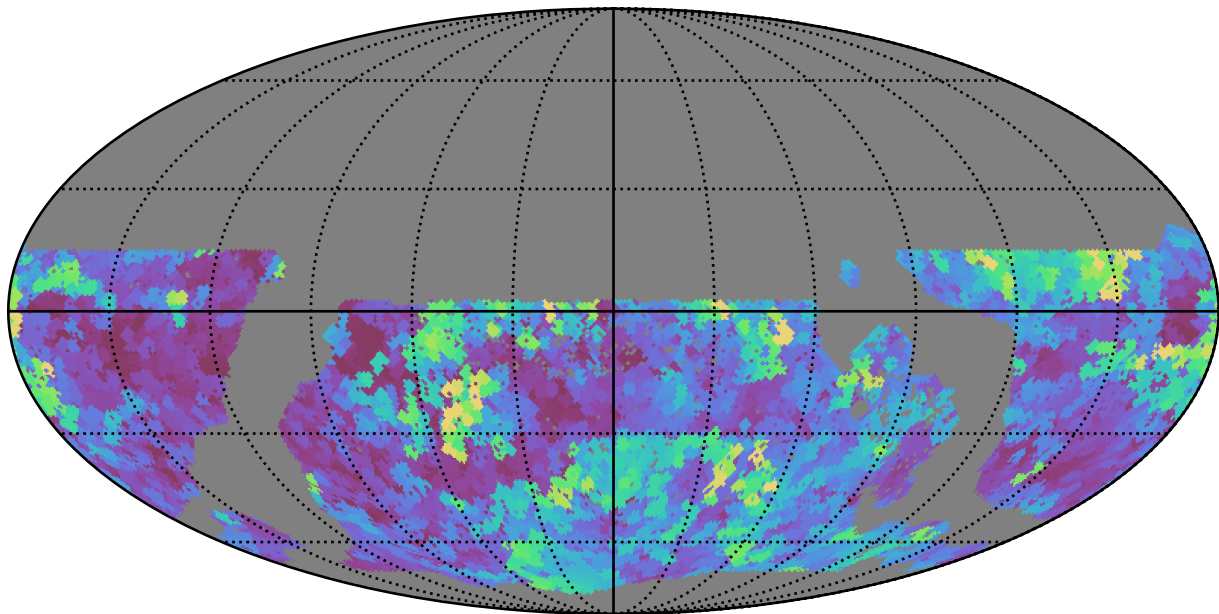
too_ignore_10_1v3.4_10yrs WFD g band: Max seeingEff
