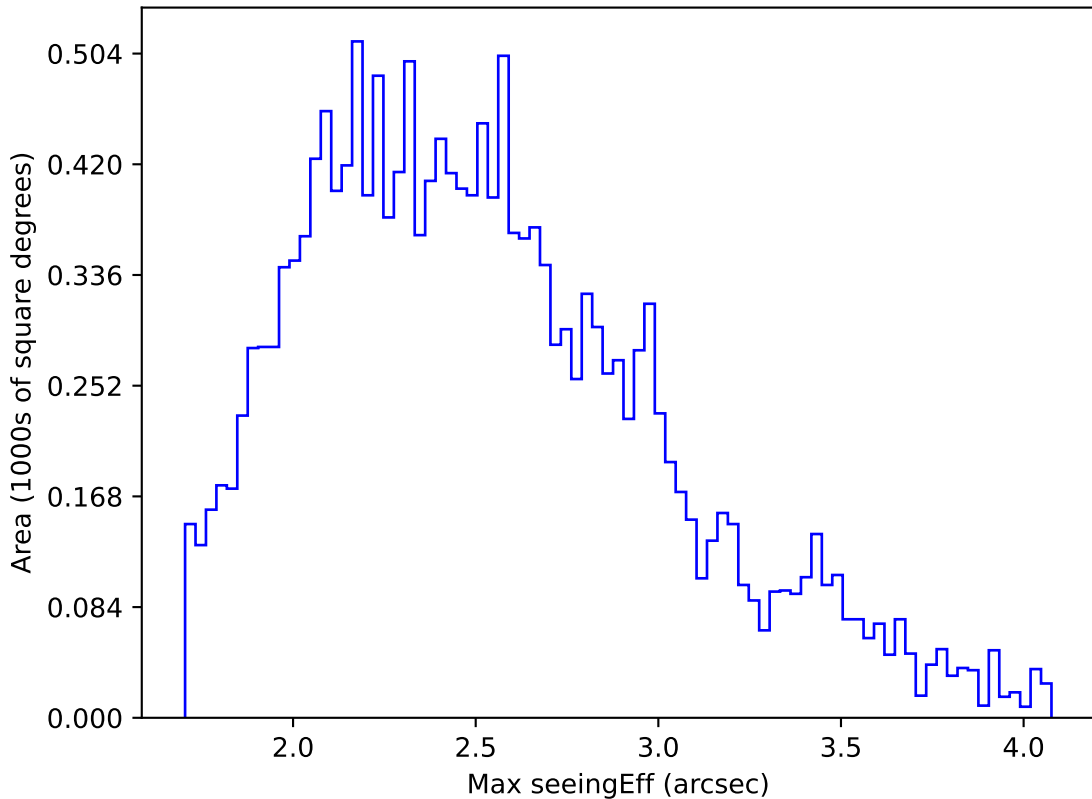
too_ignore_10_1v3.4_10yrs WFD g band: Max seeingEff
