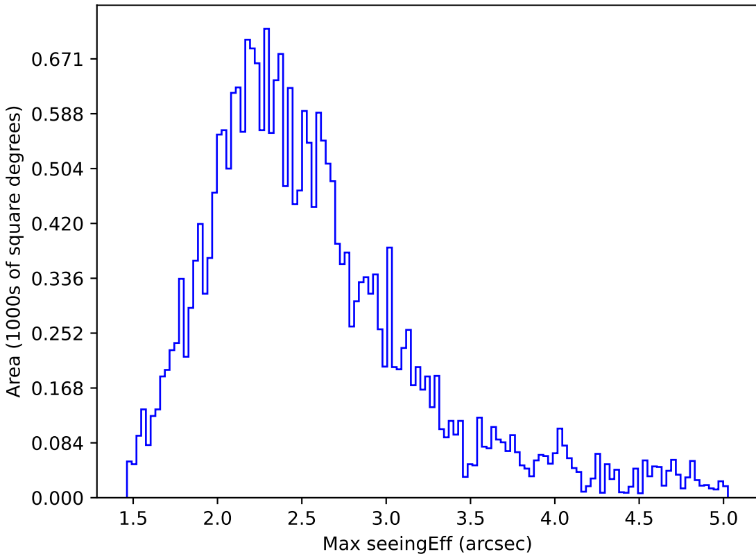
too_ignore_10_1v3.4_10yrs All sky z band: Max seeingEff
