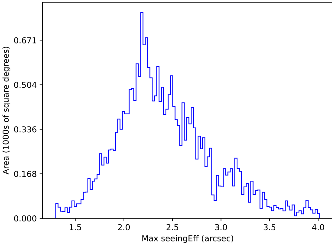
too_ignore_10_1v3.4_10yrs All sky u band: Max seeingEff
