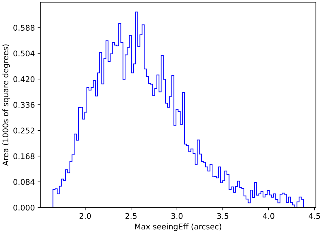
too_ignore_10_1v3.4_10yrs All sky r band: Max seeingEff
