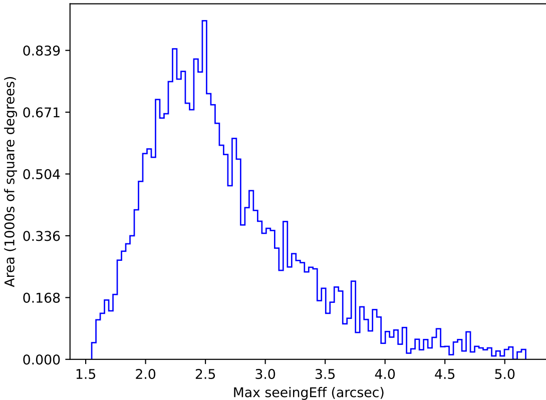
too_ignore_10_1v3.4_10yrs All sky i band: Max seeingEff
