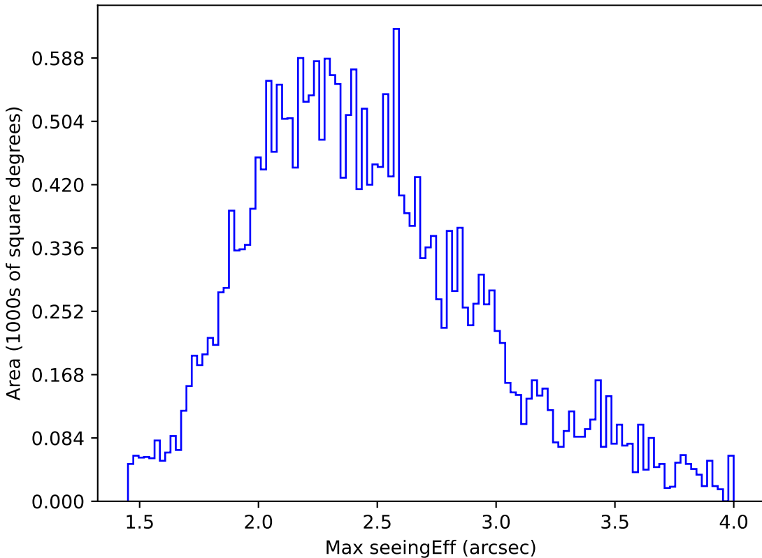
too_ignore_10_1v3.4_10yrs All sky g band: Max seeingEff
