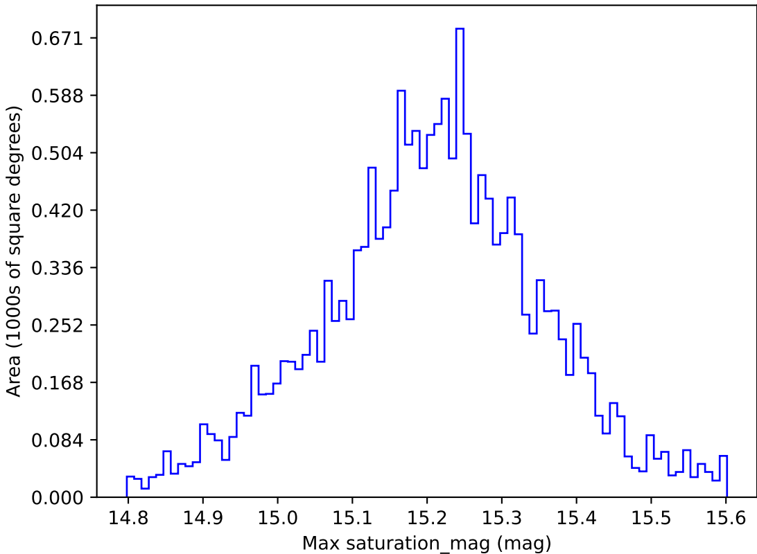
too_ignore_10_1v3.4_10yrs WFD z band: Max saturation_mag
