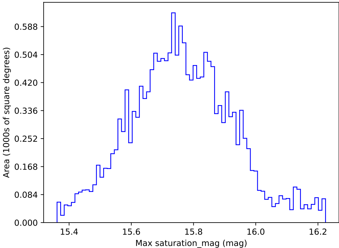
too_ignore_10_1v3.4_10yrs WFD r band: Max saturation_mag
