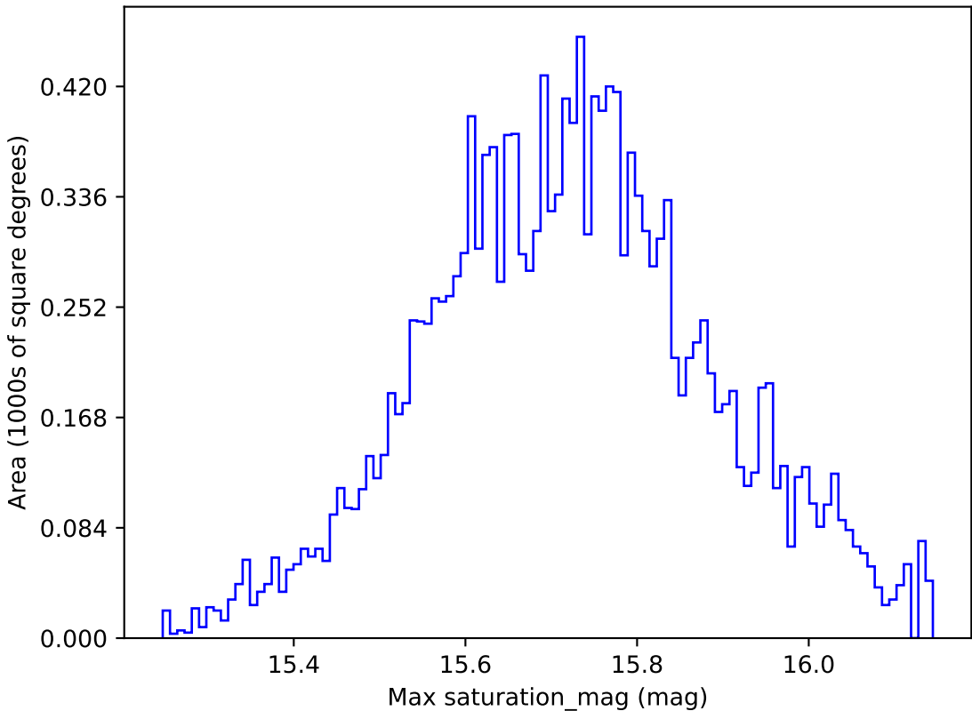
too_ignore_10_1v3.4_10yrs WFD g band: Max saturation_mag
