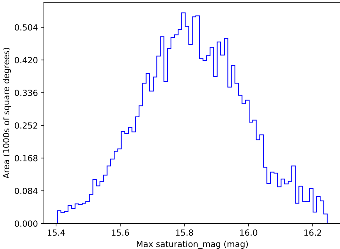
too_ignore_10_1v3.4_10yrs WFD all bands: Max saturation_mag
