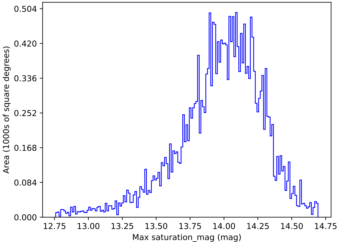
too_ignore_10_1v3.4_10yrs All sky u band: Max saturation_mag
