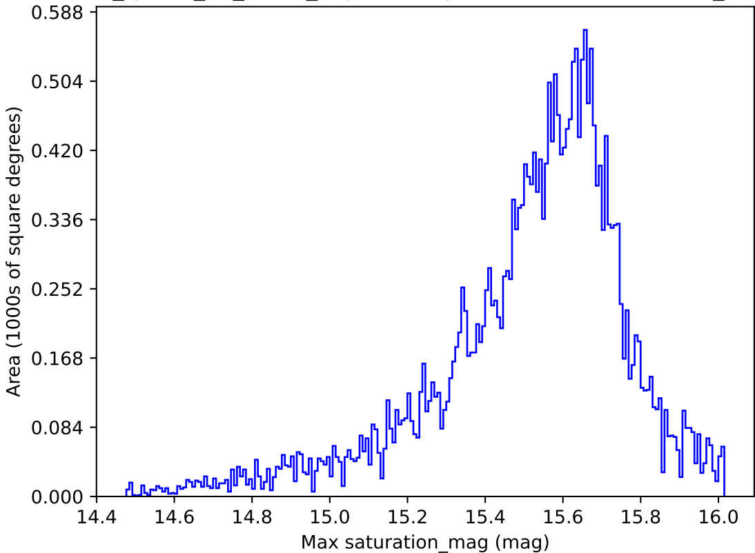
too_ignore_10_1v3.4_10yrs All sky i band: Max saturation_mag
