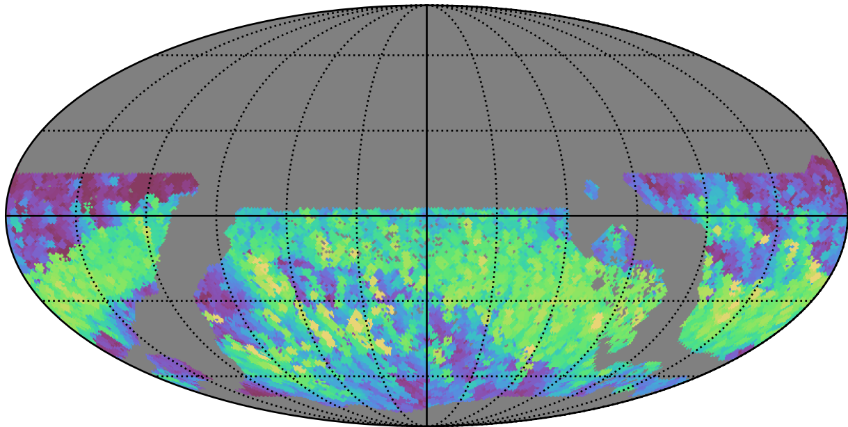
too_ignore_10_1v3.4_10yrs WFD r band: Max normairmass
