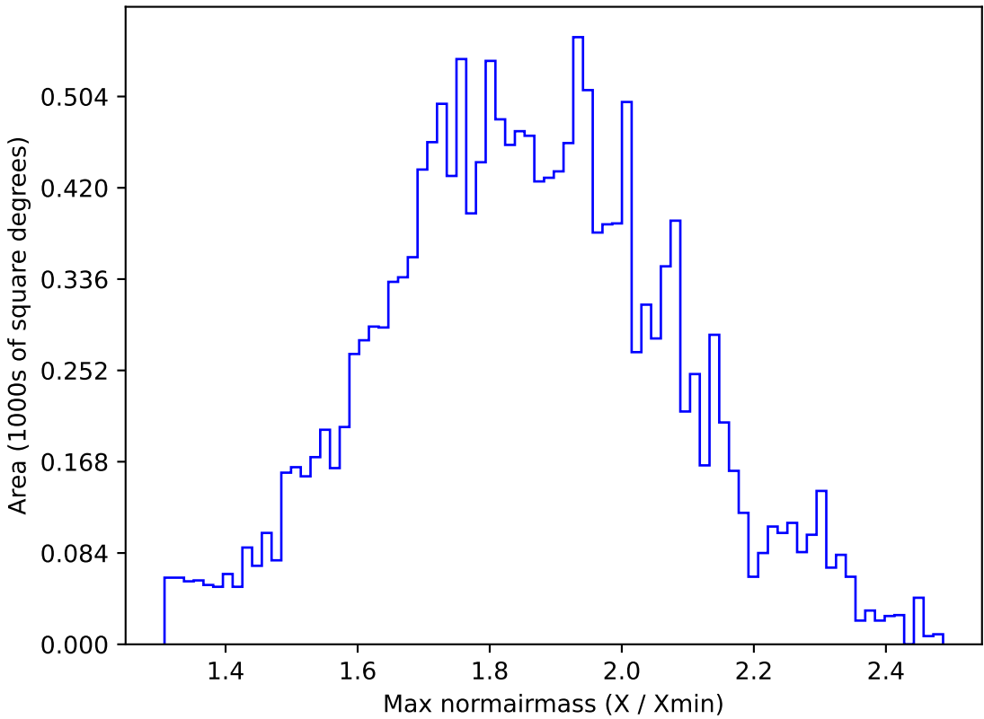
too_ignore_10_1v3.4_10yrs WFD g band: Max normairmass
