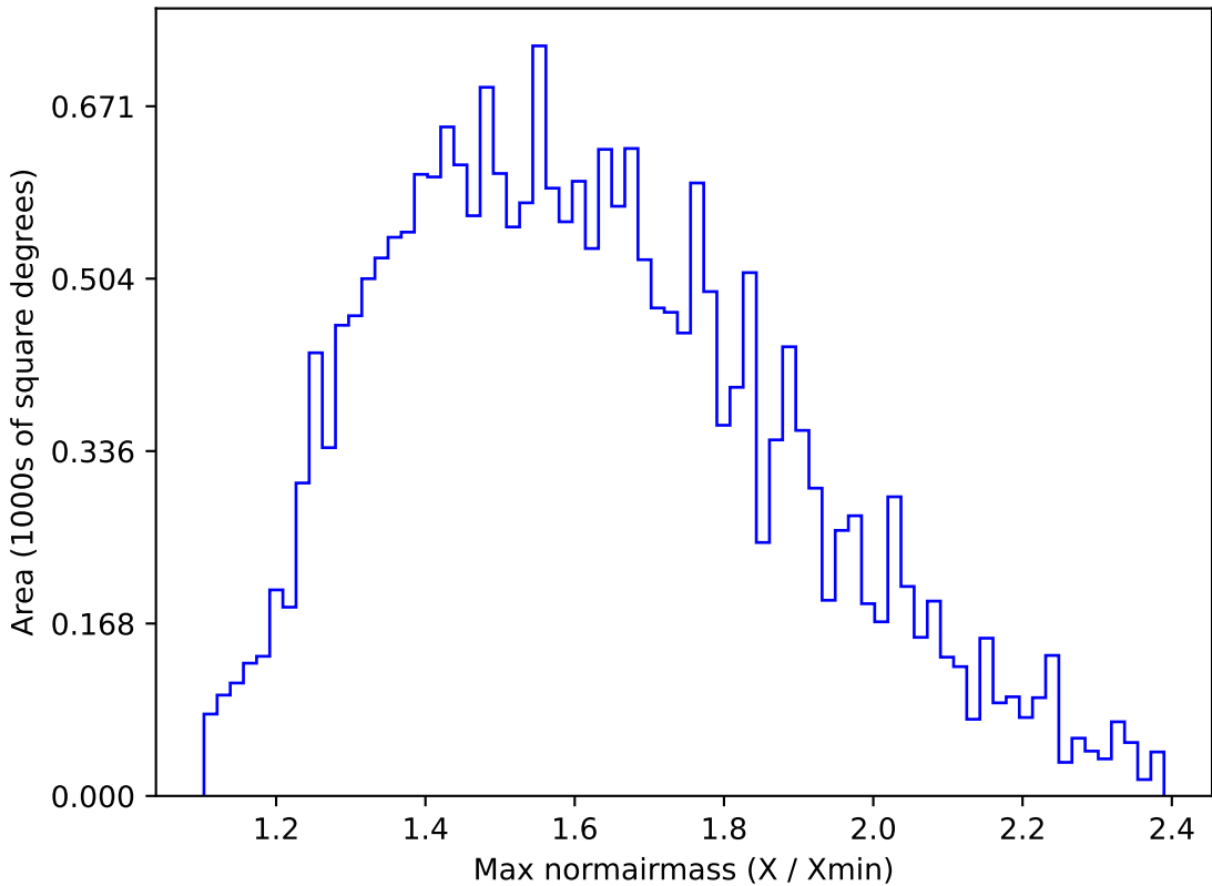
too_ignore_10_1v3.4_10yrs All sky u band: Max normairmass
