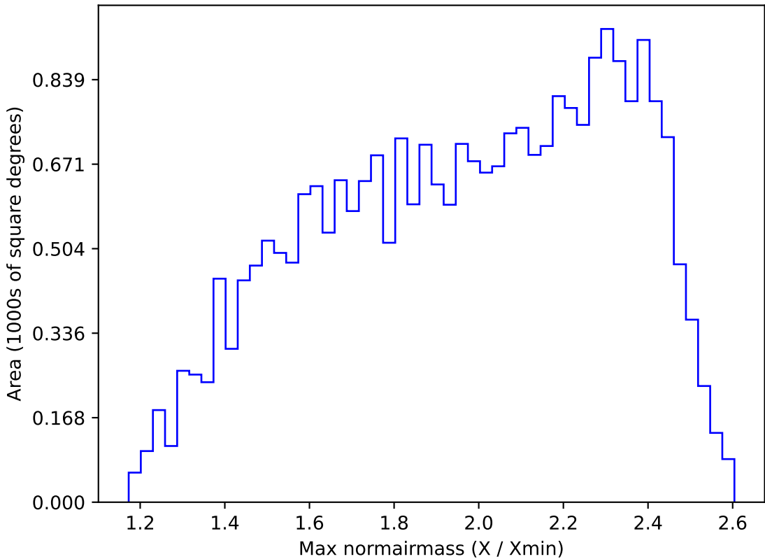
too_ignore_10_1v3.4_10yrs All sky r band: Max normairmass
