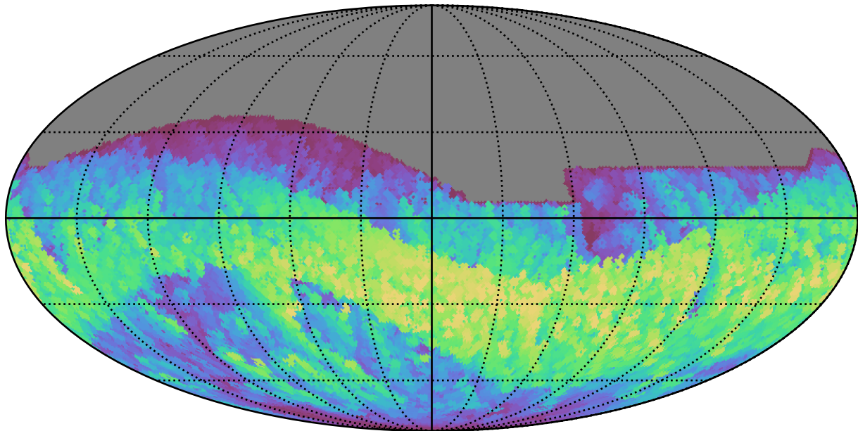
too_ignore_10_1v3.4_10yrs All sky i band: Max normairmass
