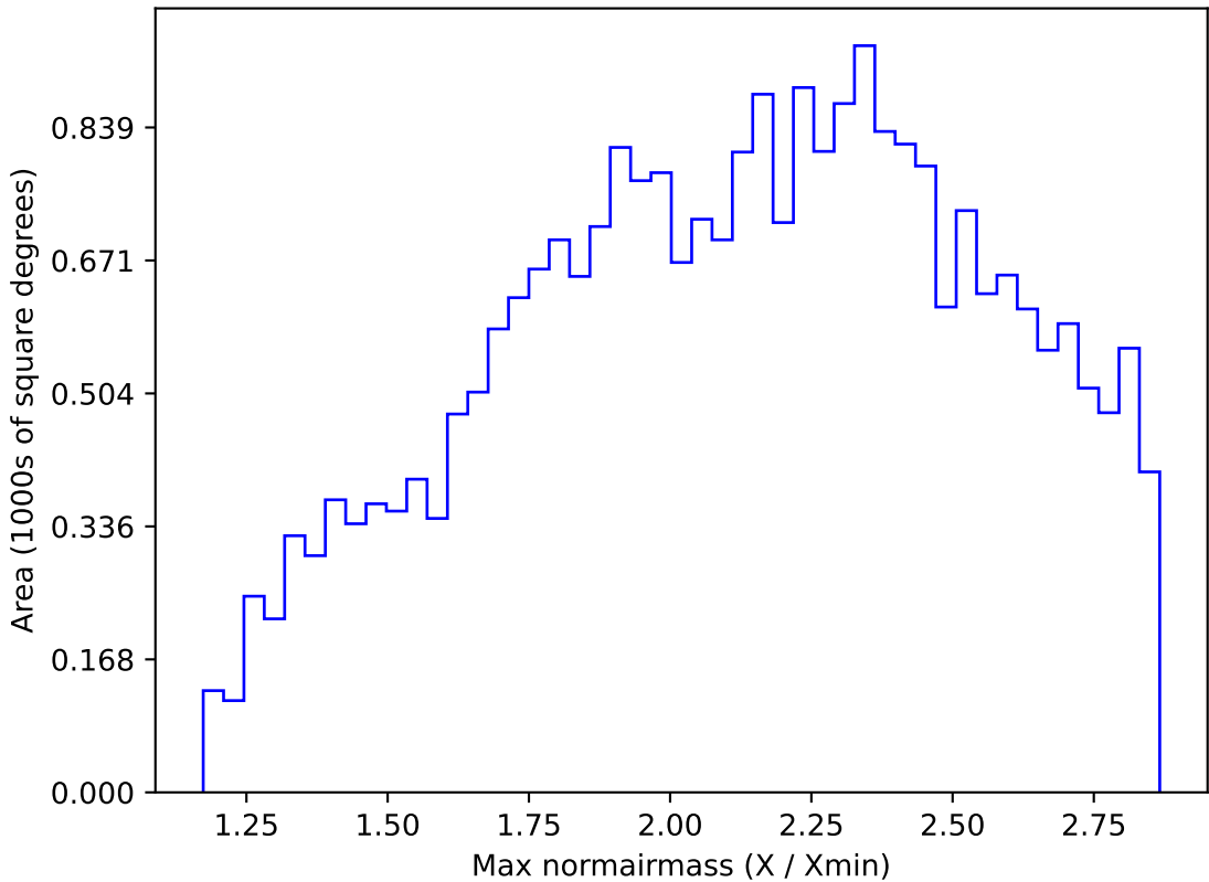
too_ignore_10_1v3.4_10yrs All sky i band: Max normairmass
