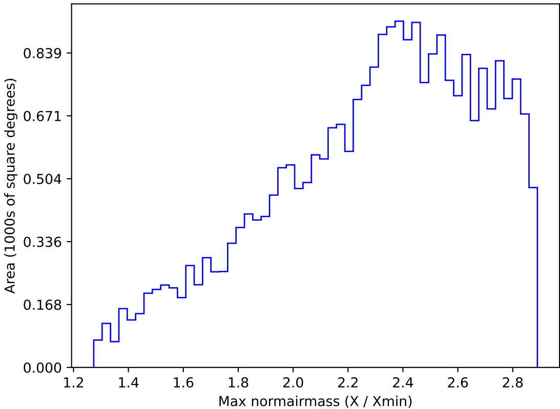
too_ignore_10_1v3.4_10yrs All sky all bands: Max normairmass
