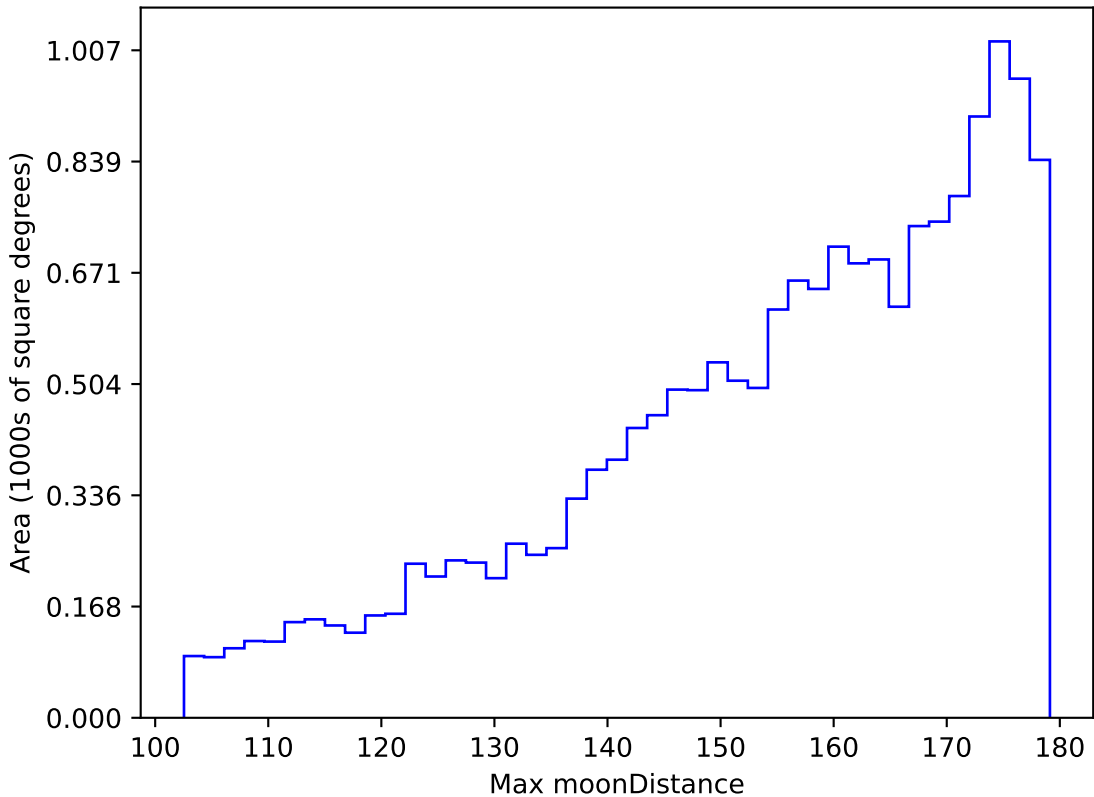
too_ignore_10_1v3.4_10yrs WFD u band: Max moonDistance
