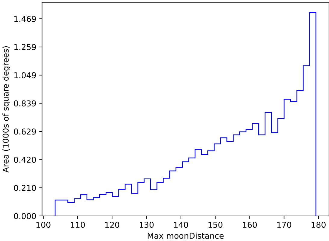
too_ignore_10_1v3.4_10yrs WFD i band: Max moonDistance
