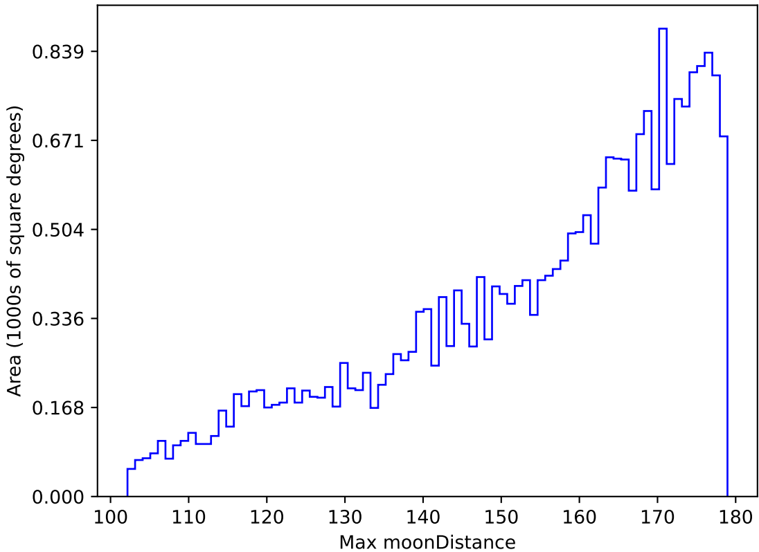
too_ignore_10_1v3.4_10yrs All sky z band: Max moonDistance
