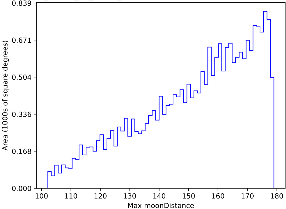
too_ignore_10_1v3.4_10yrs All sky u band: Max moonDistance
