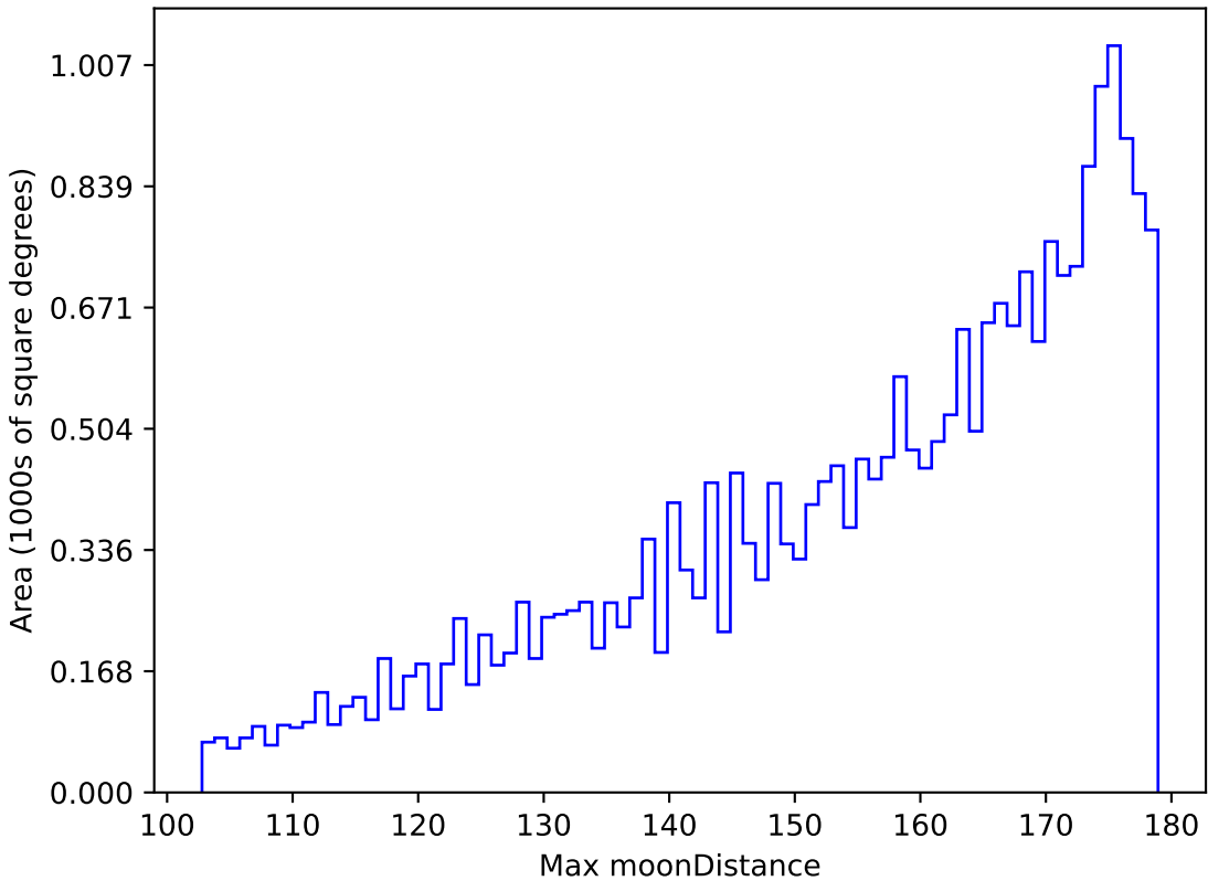
too_ignore_10_1v3.4_10yrs All sky g band: Max moonDistance
