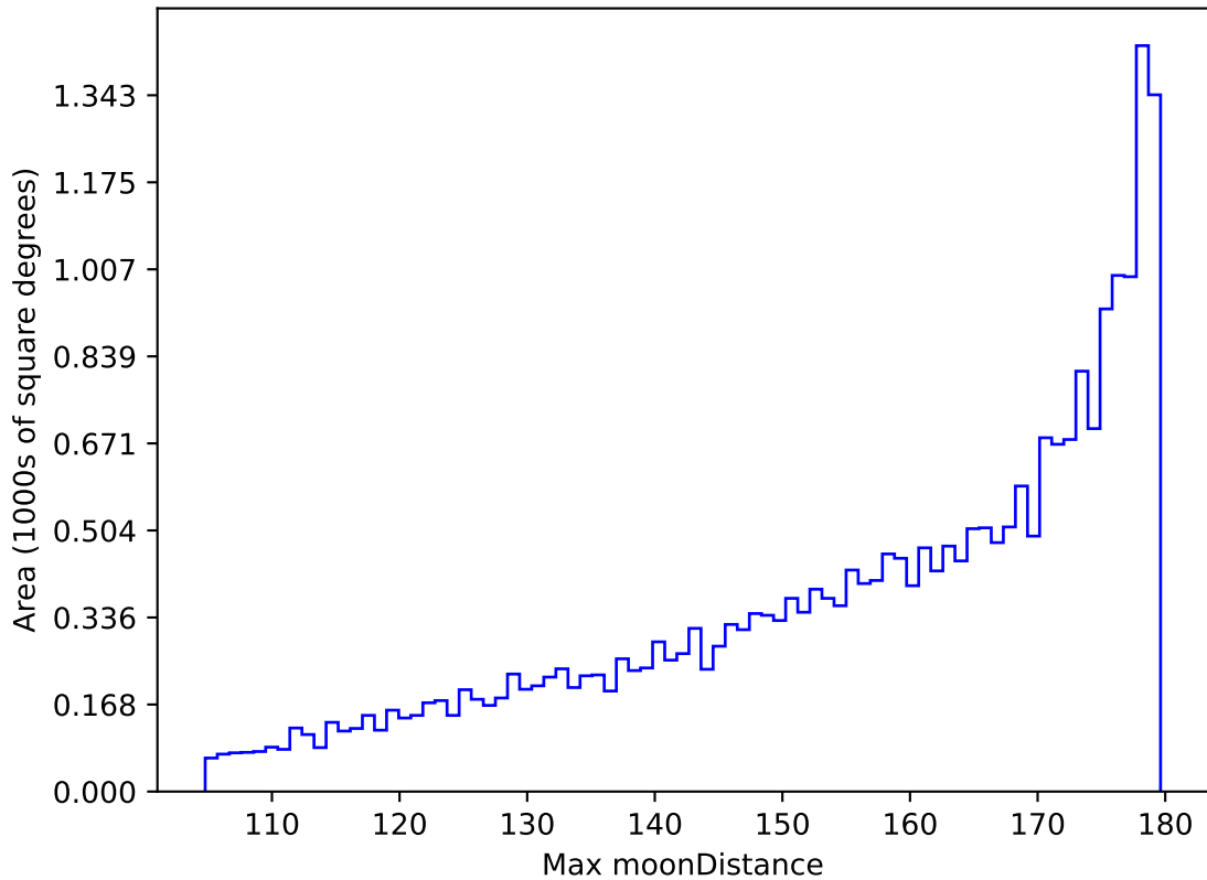
too_ignore_10_1v3.4_10yrs All sky all bands: Max moonDistance
