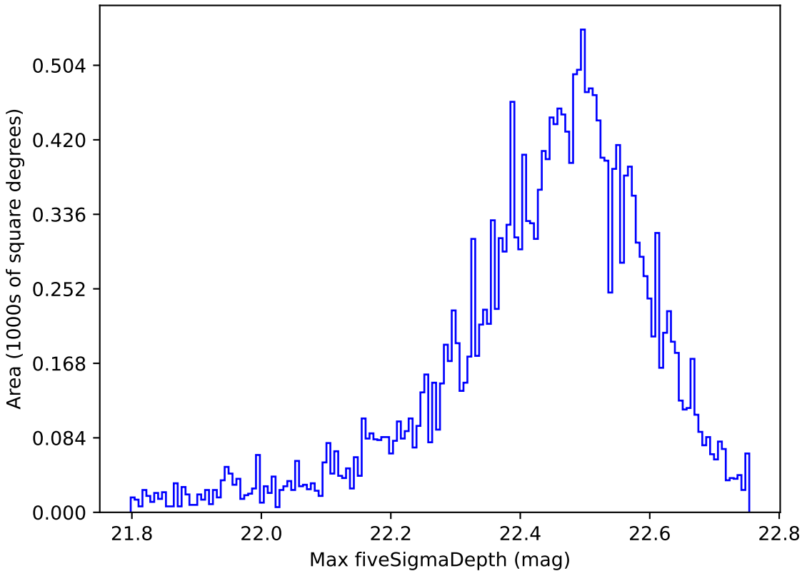
too_ignore_10_1v3.4_10yrs Yr 1 y band: Max fiveSigmaDepth
