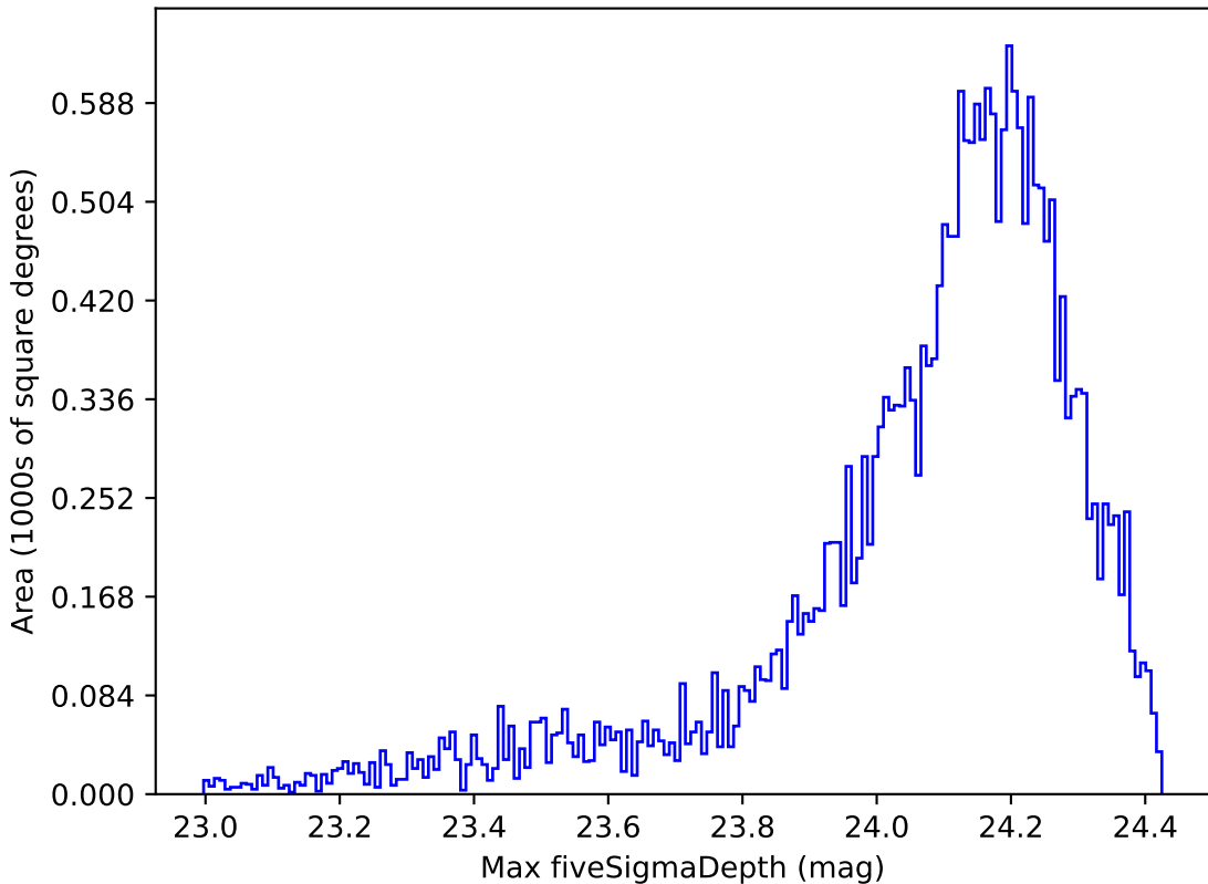
too_ignore_10_1v3.4_10yrs Yr 1 i band: Max fiveSigmaDepth
