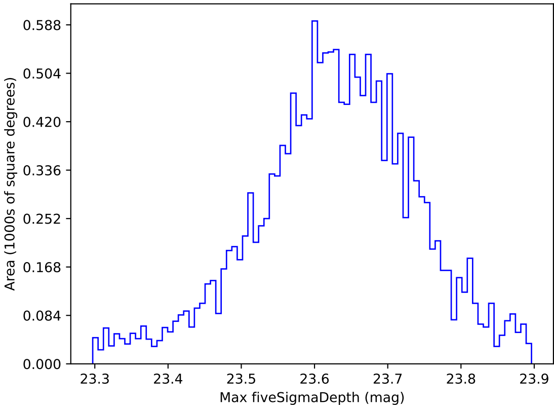
too_ignore_10_1v3.4_10yrs WFD z band: Max fiveSigmaDepth
